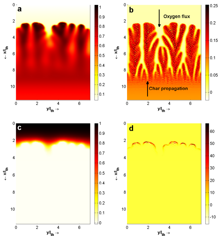
FIGURE 7. Macroscopic profiles of the spatial structure of the flame front: (a) Temperature T^0 , (b) Reaction product \mathcal{R}^0 , (c) Active concentration C^0 , (d) Heat released rate W(C^0, T^0) .
